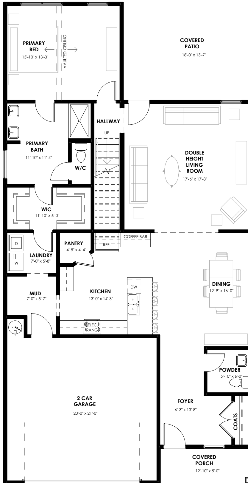
LEVEL 1 FLOOR PLAN
