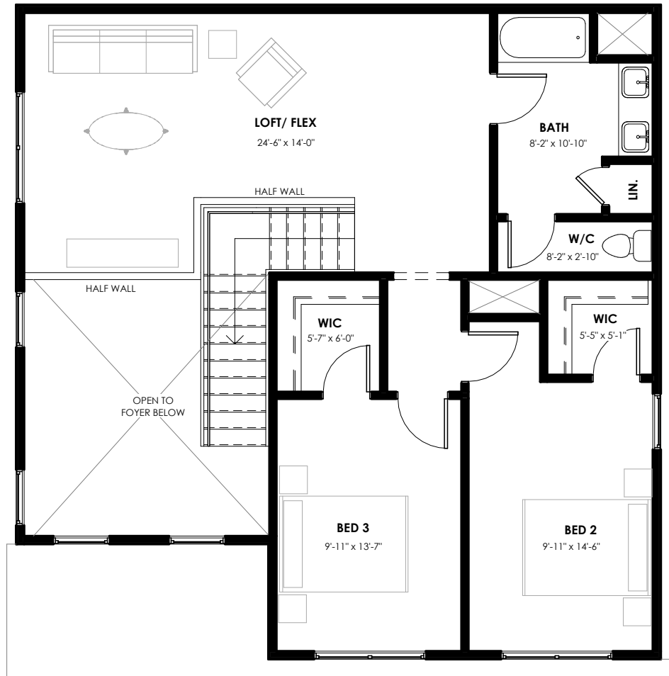
LEVEL 2 FLOOR PLAN
