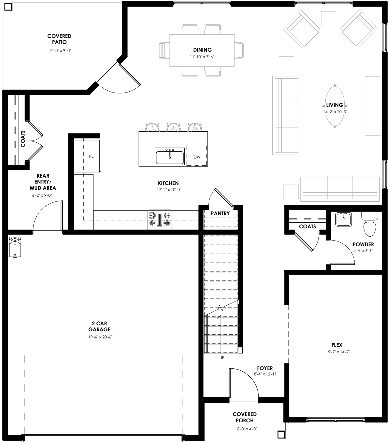
LEVEL 1 FLOOR PLAN
