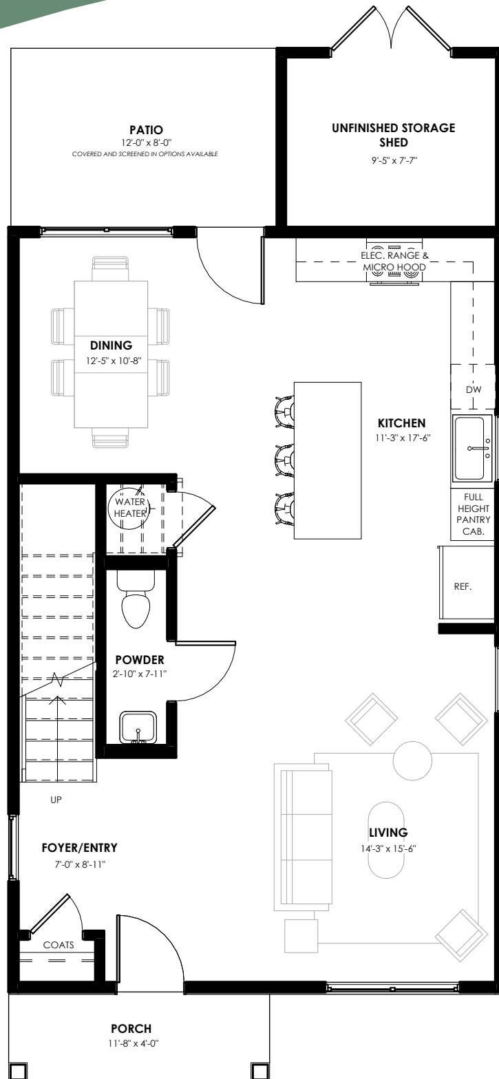
LEVEL 1 FLOOR PLAN
